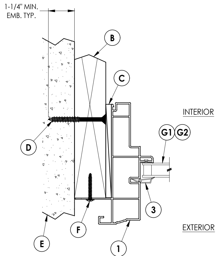
2 HORIZONTAL CROSS SECTION 2 Shown w/ 2X Buck Construction
