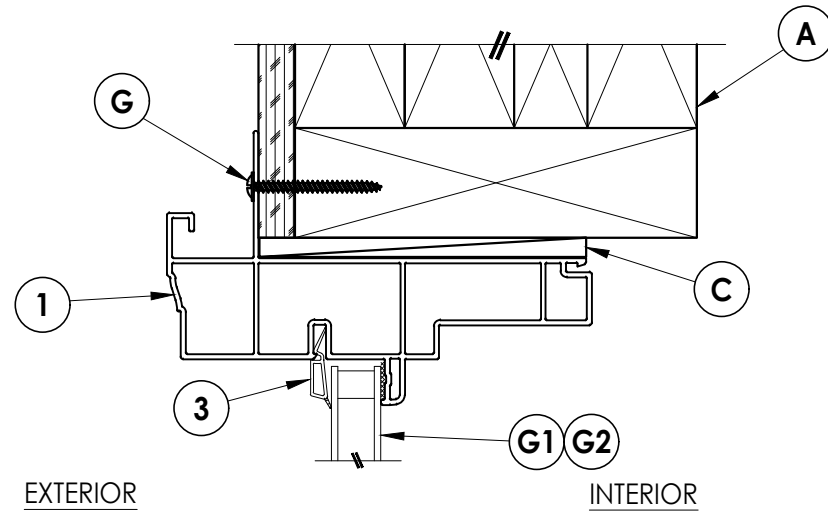
1 VERTICAL CROSS SECTION 2 Shown w/ 2X Stud Construction
